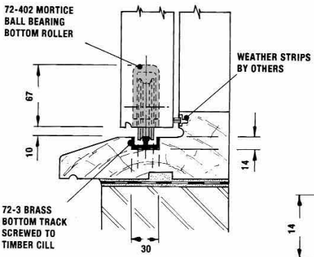
ALTERNATIVE SECTION TIMBER CILL
