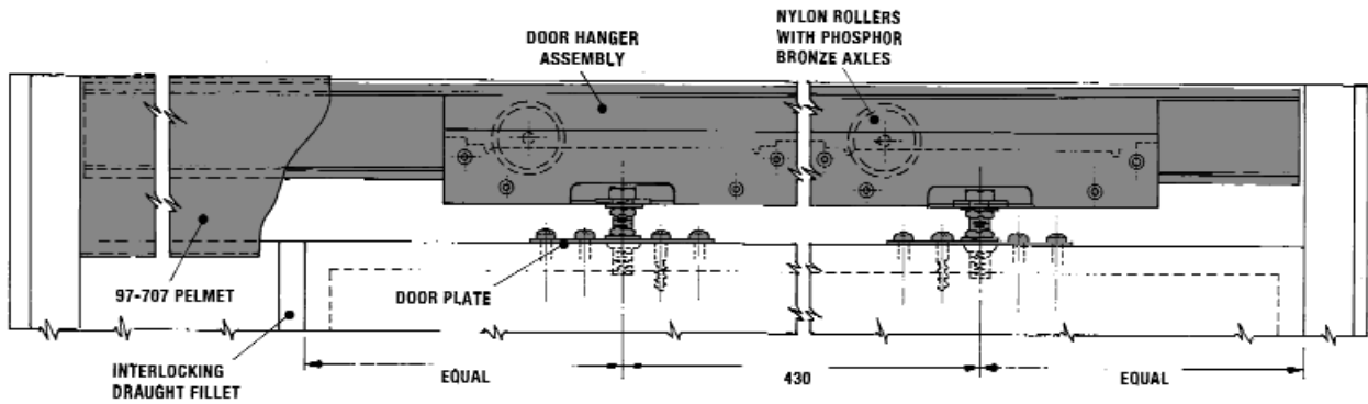
PLAN AND ELEVATION- DOOR ON FACE OF WALL
