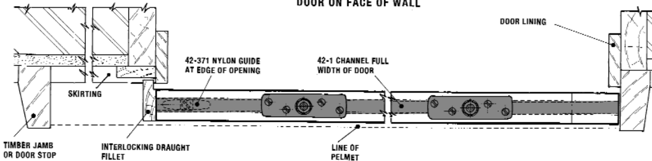
PLAN AND ELEVATION- DOOR ON FACE OF WALL
