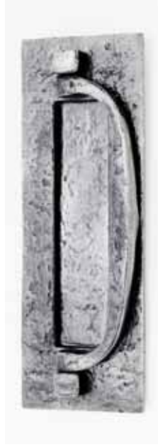
305 Postal Knocker Overall 300mm x 105mm, opening 200mm x 44mm, fixing centres 256mm
